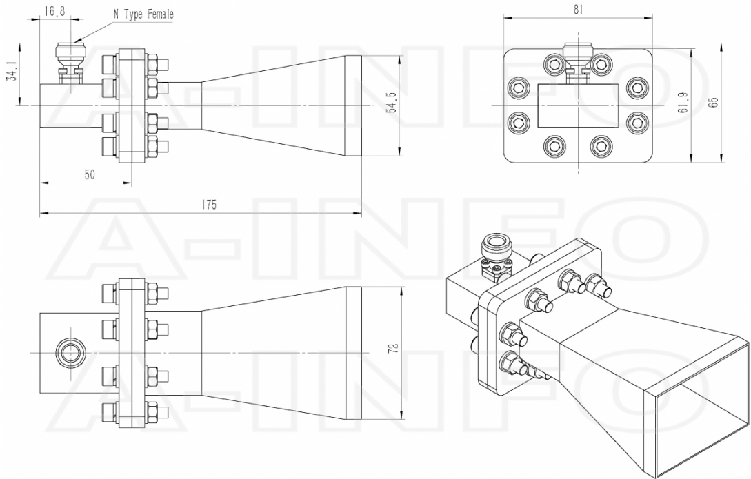
N-Female Output (P/N: LB-159-10-C-NF)
